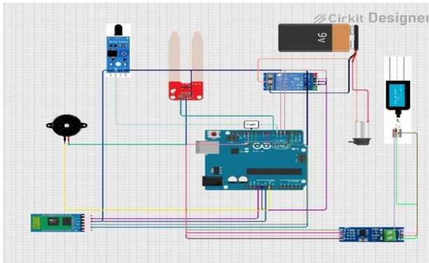
Figure 1: IOT Setup of Smart Agriculture System Using IoT and Machine Learning
